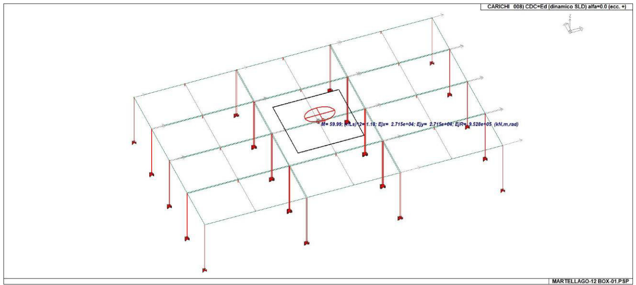
22_CDC_008_CDC=Ed (dinamico SLD) alfa=0.0 (ecc. +)
